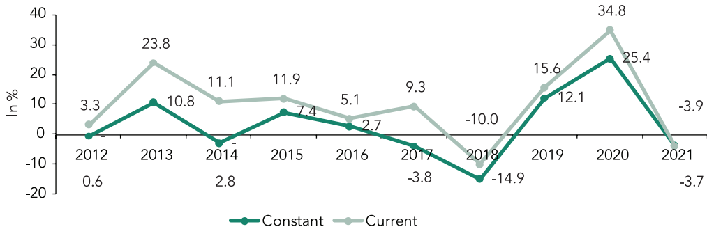
Figure 4.3 Electricity sector growth in current and constant
